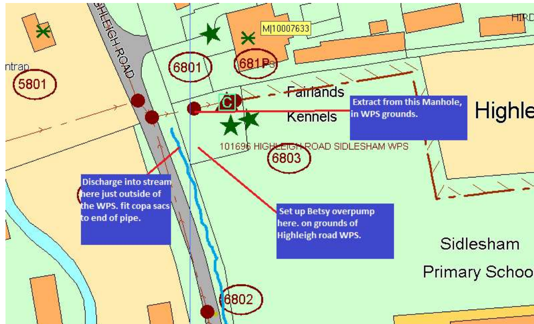
Highley Road SPS Over-pumping set up location
